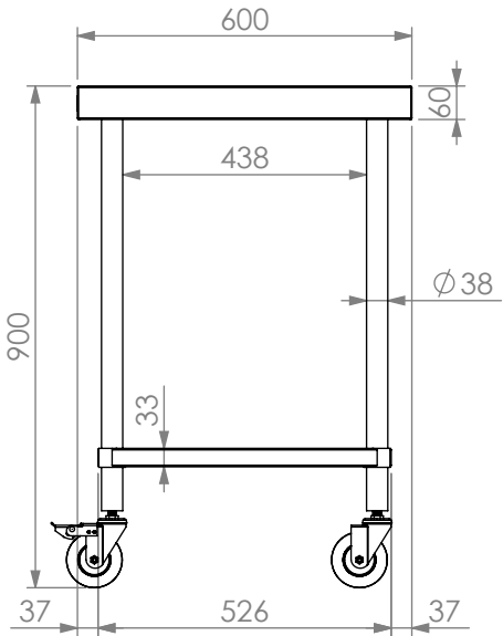
*600mm DEEP MODULE ELEVATION.
