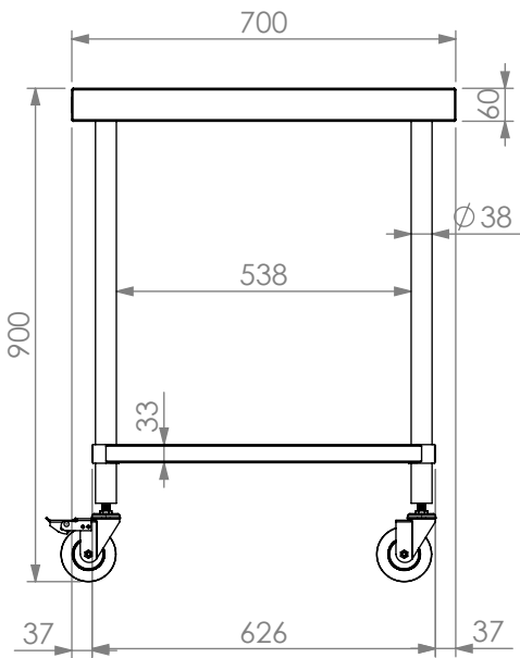
*700mm DEEP MODULE ELEVATION.
